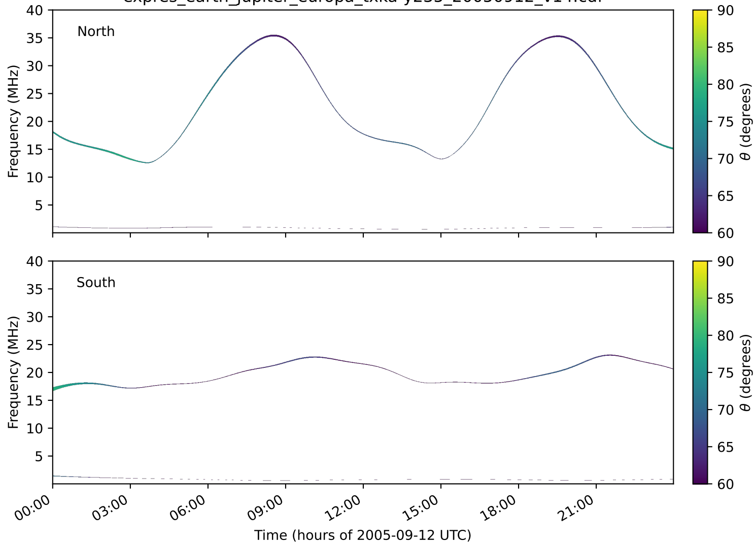
expres_earth_jupiter_europa_txka-y235_20050912_v14.cdf
