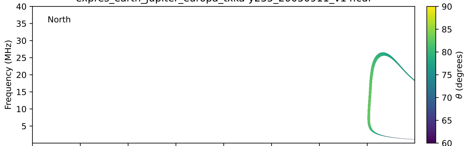
expres_earth_jupiter_europa_txka-y235_20050911_v14.cdf
