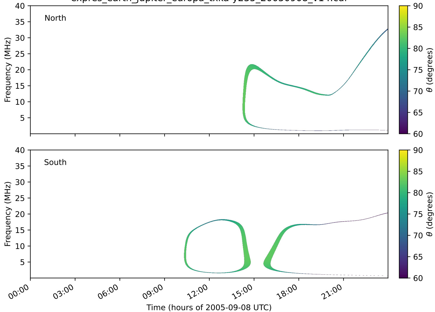
expres_earth_jupiter_europa_txka-y235_20050908_v14.cdf
