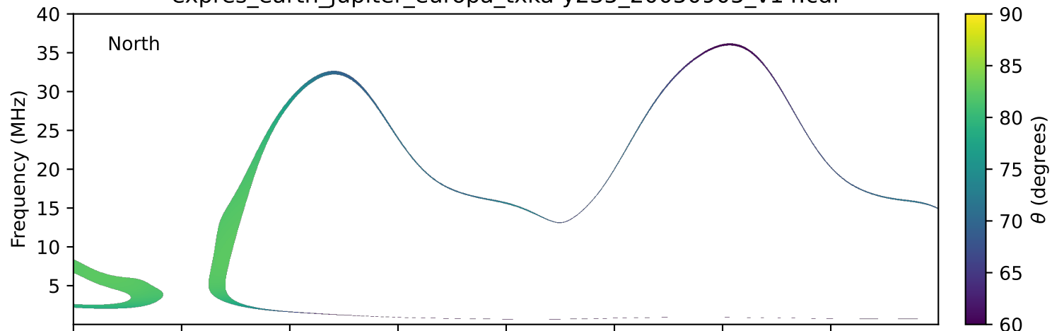
expres_earth_jupiter_europa_txka-y235_20050905_v14.cdf
