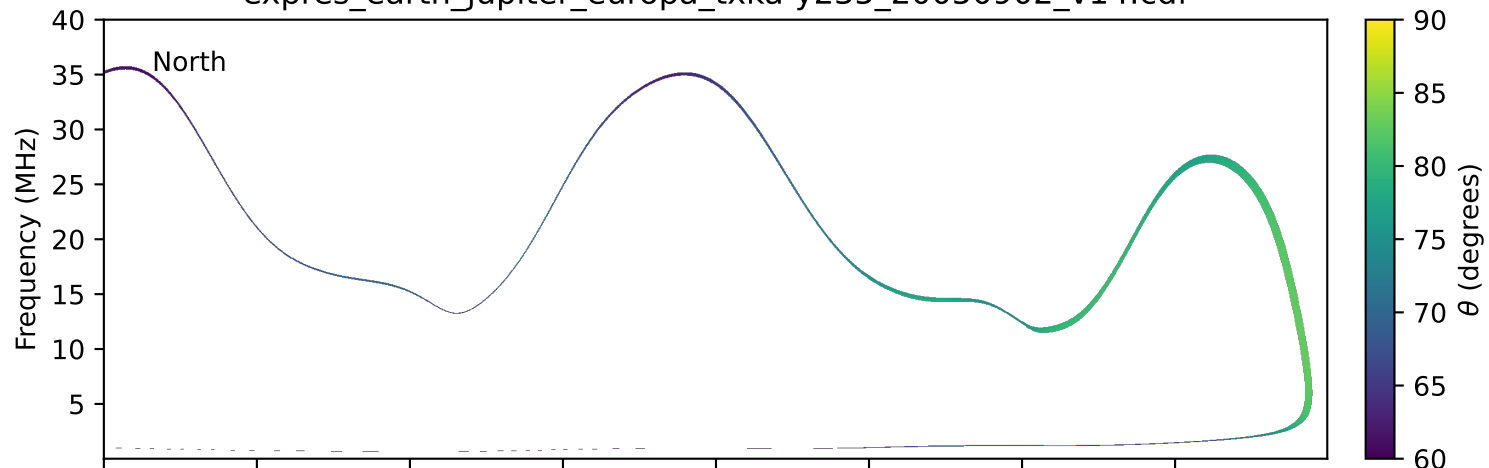
expres_earth_jupiter_europa_txka-y235_20050902_v14.cdf
