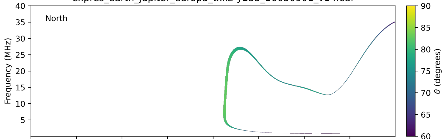
expres_earth_jupiter_europa_txka-y235_20050901_v14.cdf
