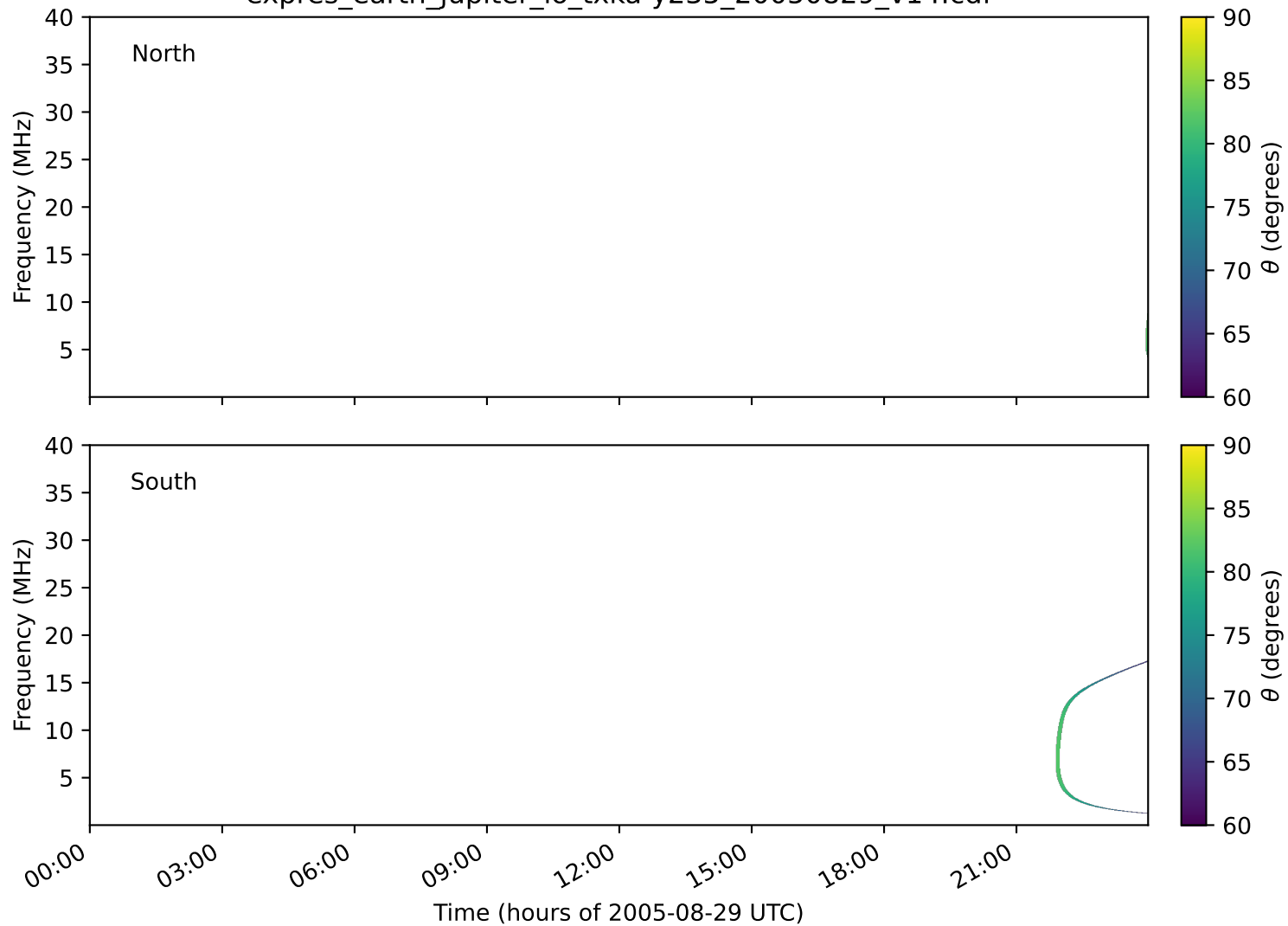
expres_earth_jupiter_io_txka-y235_20050829_v14.cdf
