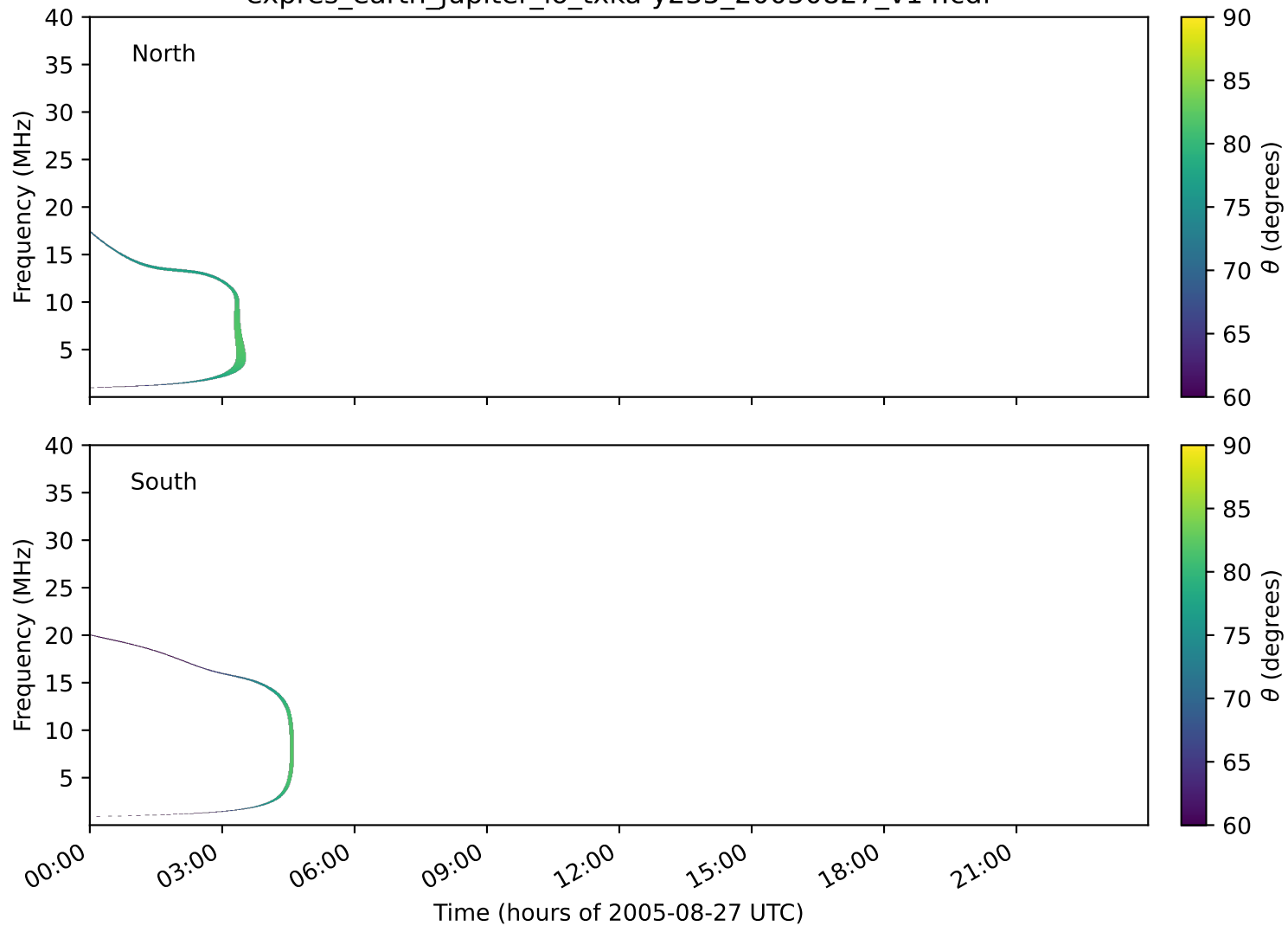
expres_earth_jupiter_io_txka-y235_20050827_v14.cdf
