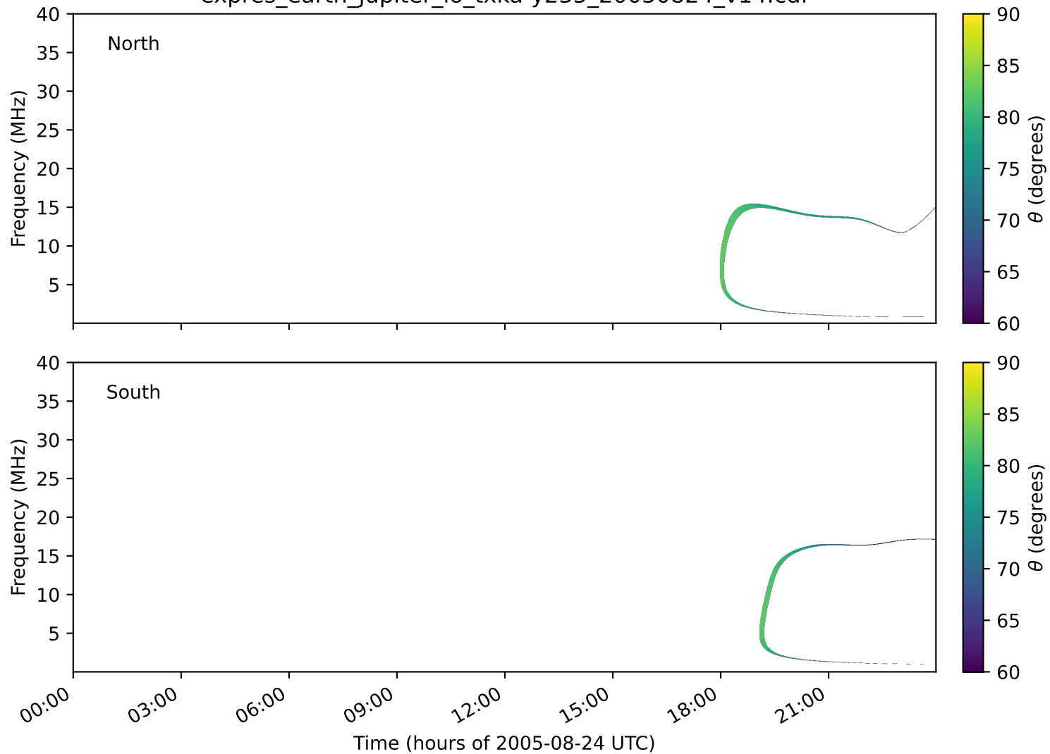
expres_earth_jupiter_io_txka-y235_20050824_v14.cdf
