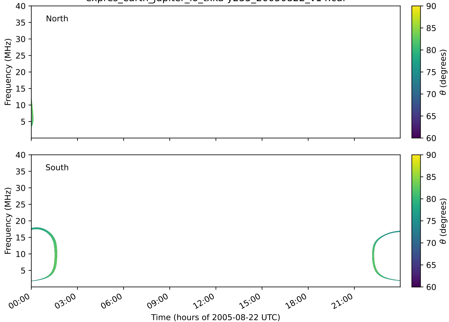
expres_earth_jupiter_io_txka-y235_20050822_v14.cdf
