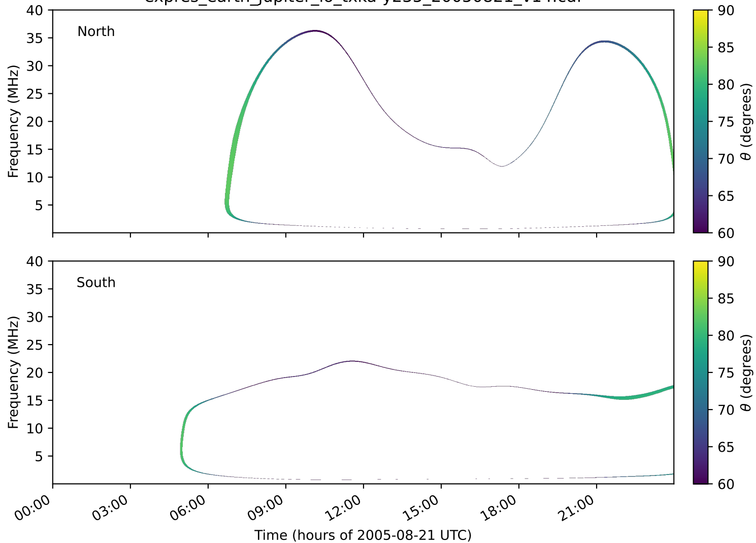
expres_earth_jupiter_io_txka-y235_20050821_v14.cdf
