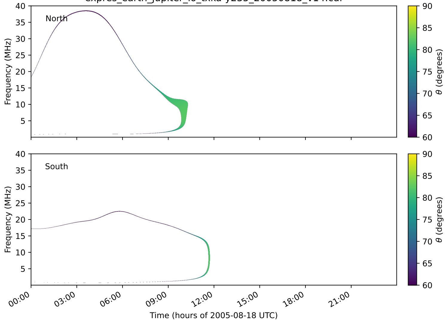
expres_earth_jupiter_io_txka-y235_20050818_v14.cdf
