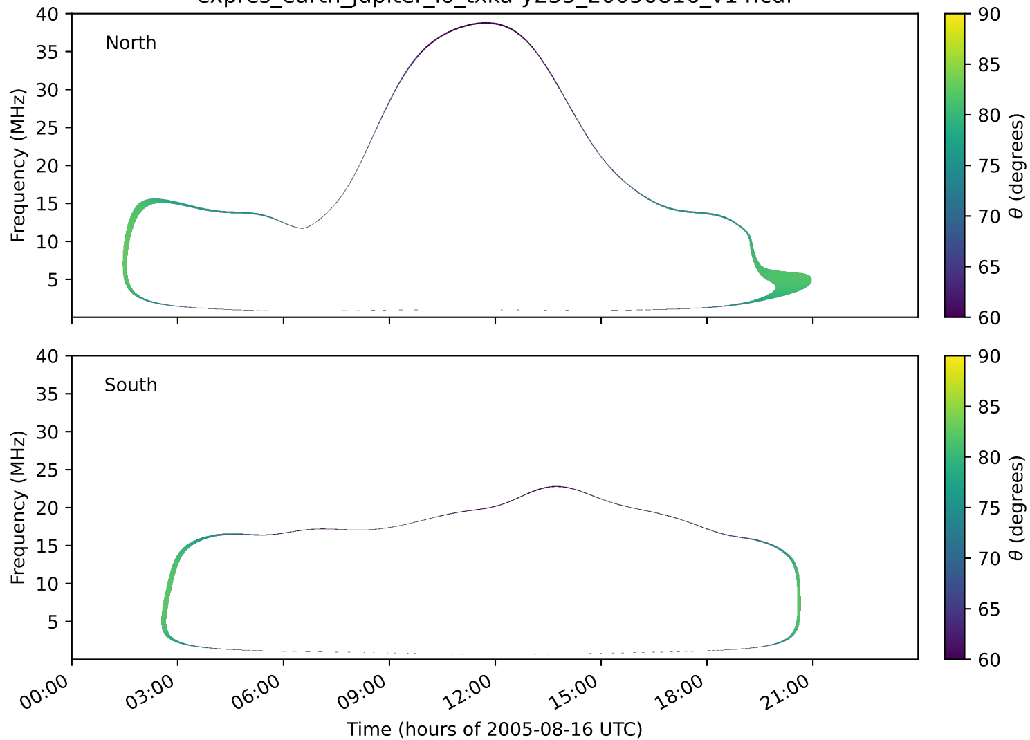
expres_earth_jupiter_io_txka-y235_20050816_v14.cdf
