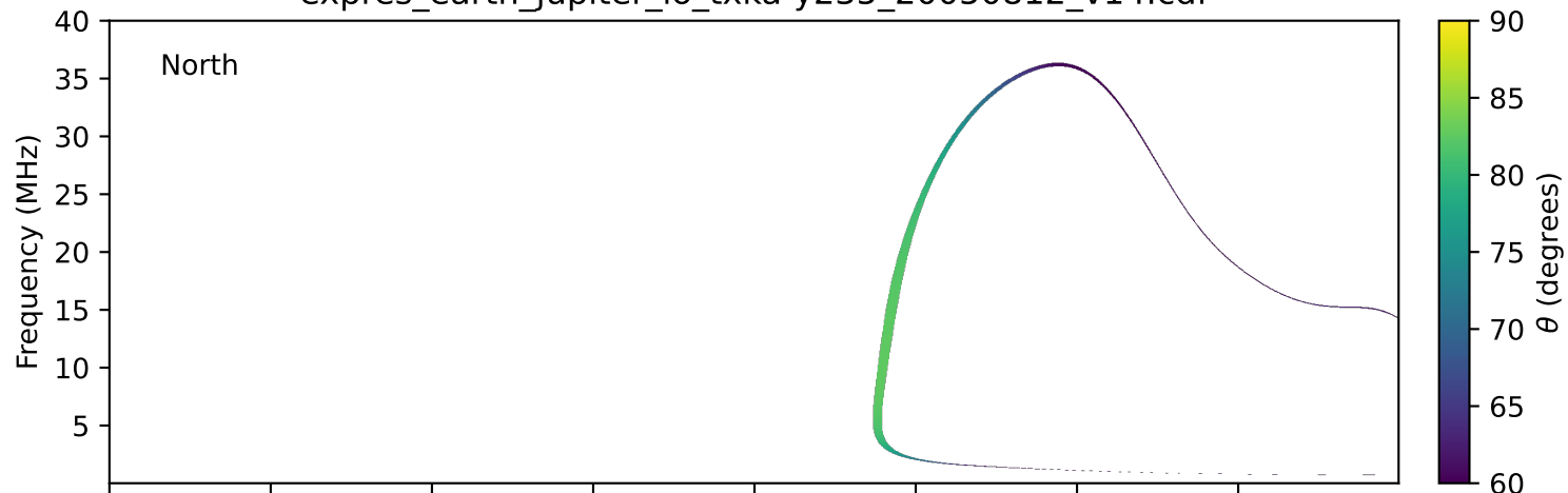
expres_earth_jupiter_io_txka-y235_20050812_v14.cdf
