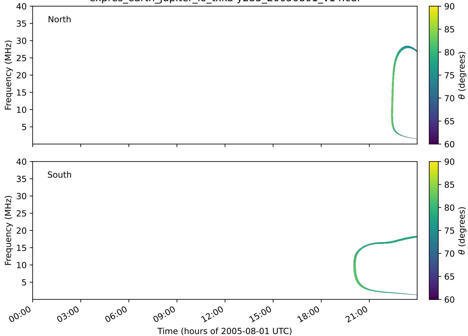
expres_earth_jupiter_io_txka-y235_20050801_v14.cdf
