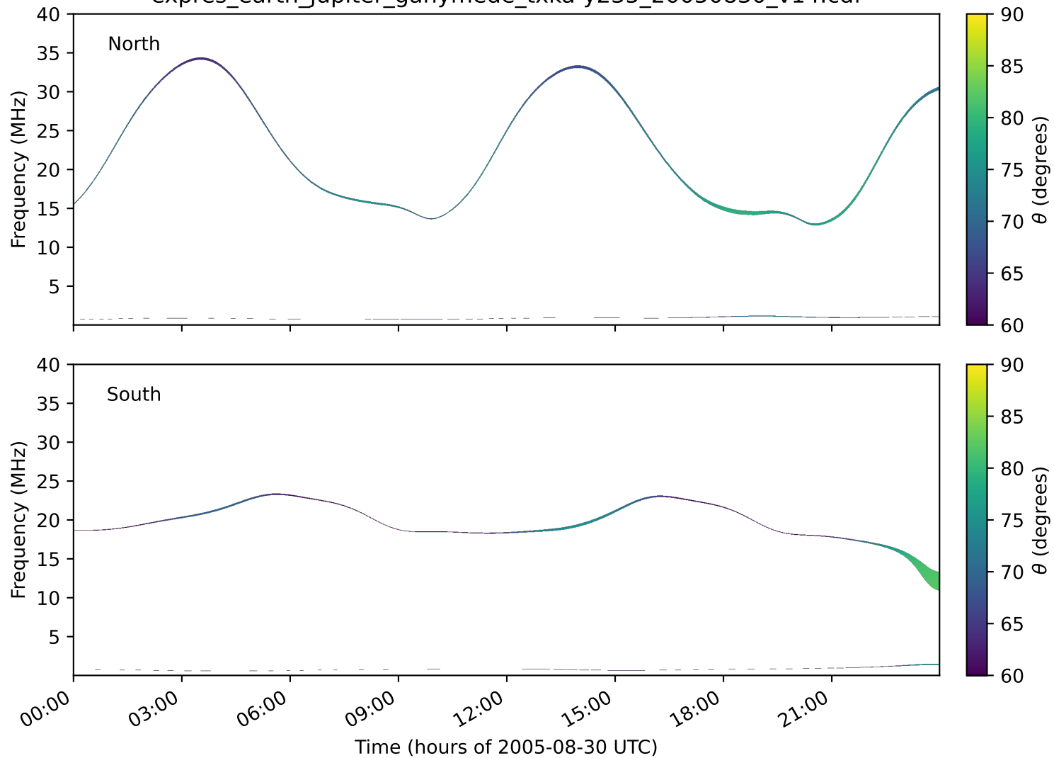
expres_earth_jupiter_ganymede_txka-y235_20050830_v14.cdf
