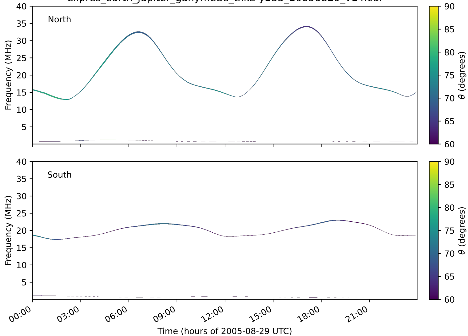
expres_earth_jupiter_ganymede_txka-y235_20050829_v14.cdf
