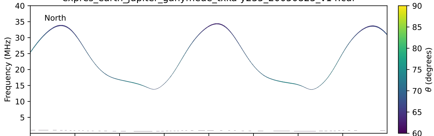
expres_earth_jupiter_ganymede_txka-y235_20050823_v14.cdf
