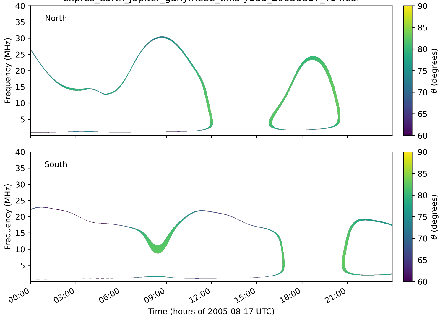
expres_earth_jupiter_ganymede_txka-y235_20050817_v14.cdf
