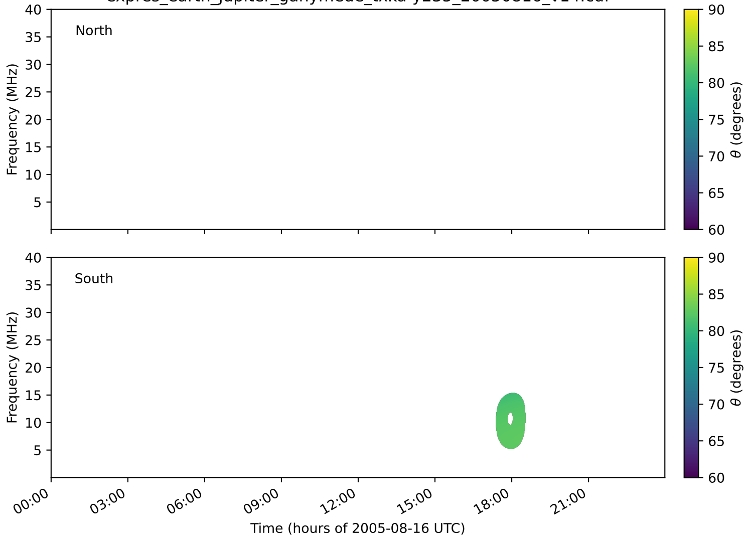
expres_earth_jupiter_ganymede_txka-y235_20050816_v14.cdf
