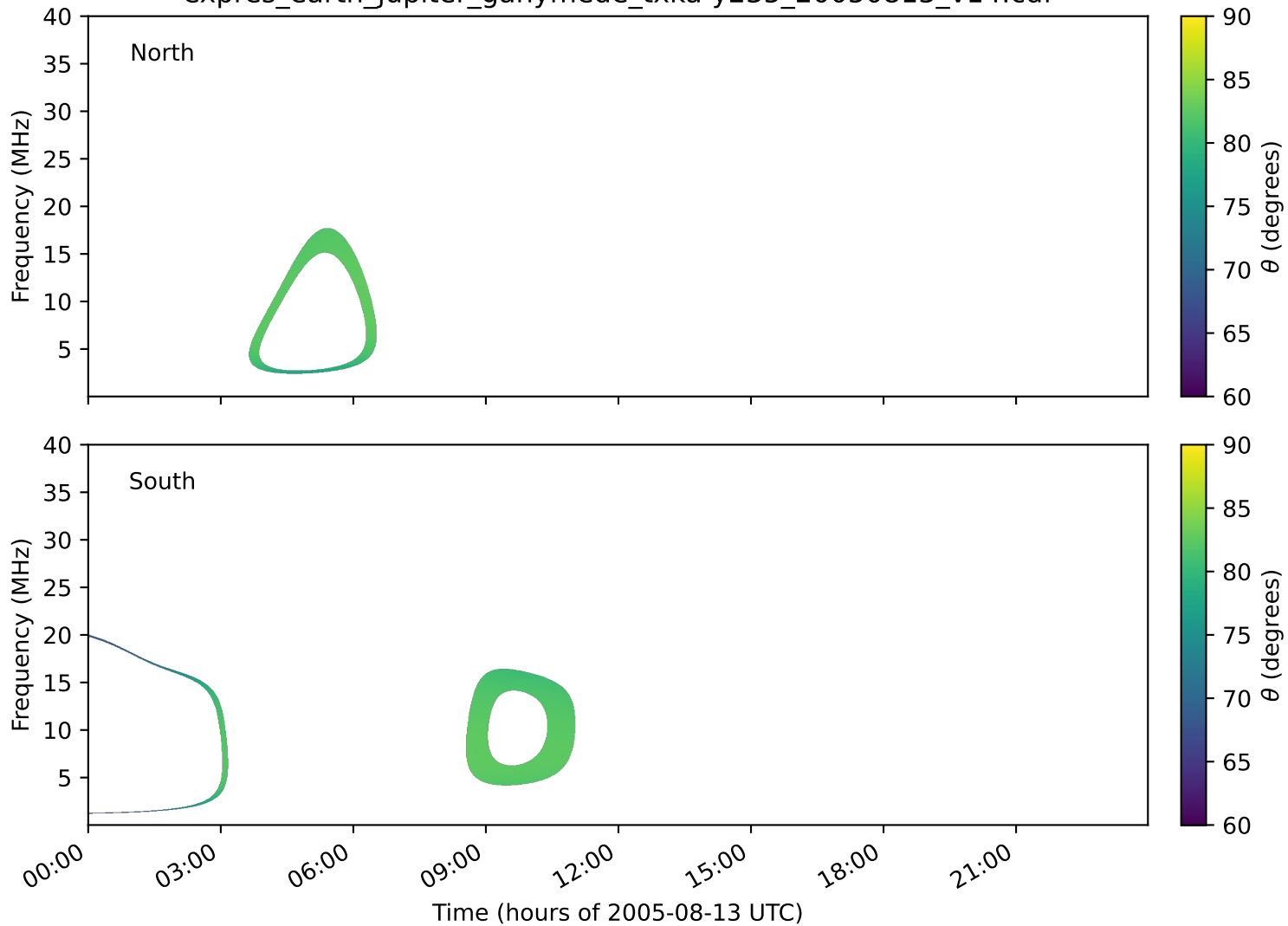
expres_earth_jupiter_ganymede_txka-y235_20050813_v14.cdf
