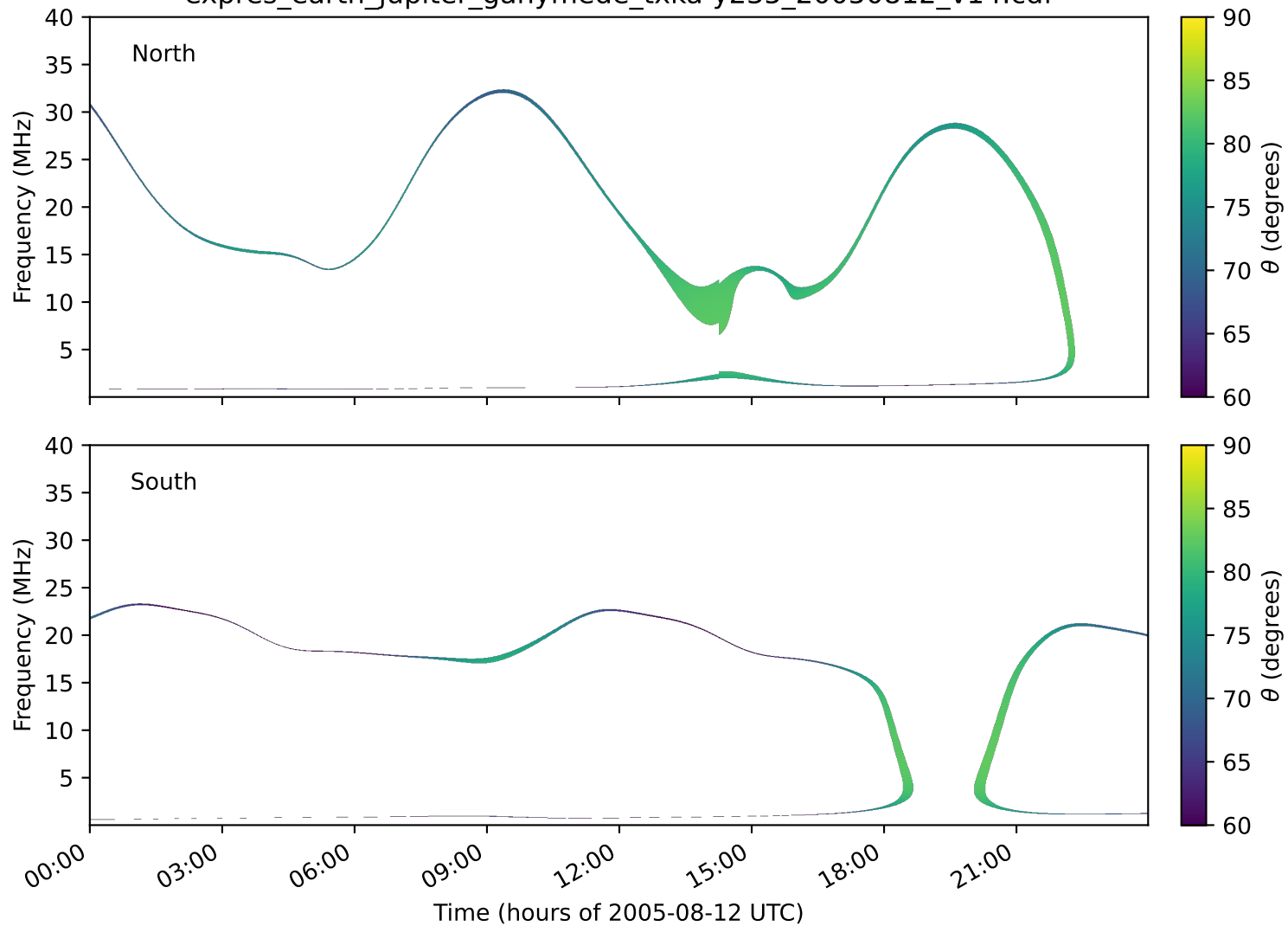
expres_earth_jupiter_ganymede_txka-y235_20050812_v14.cdf
