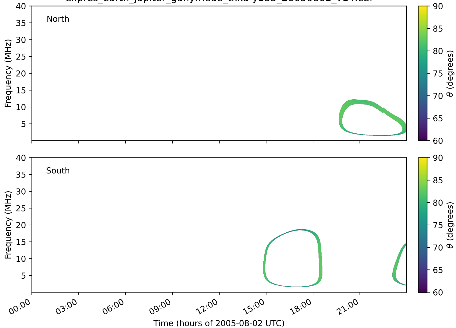
expres_earth_jupiter_ganymede_txka-y235_20050802_v14.cdf
