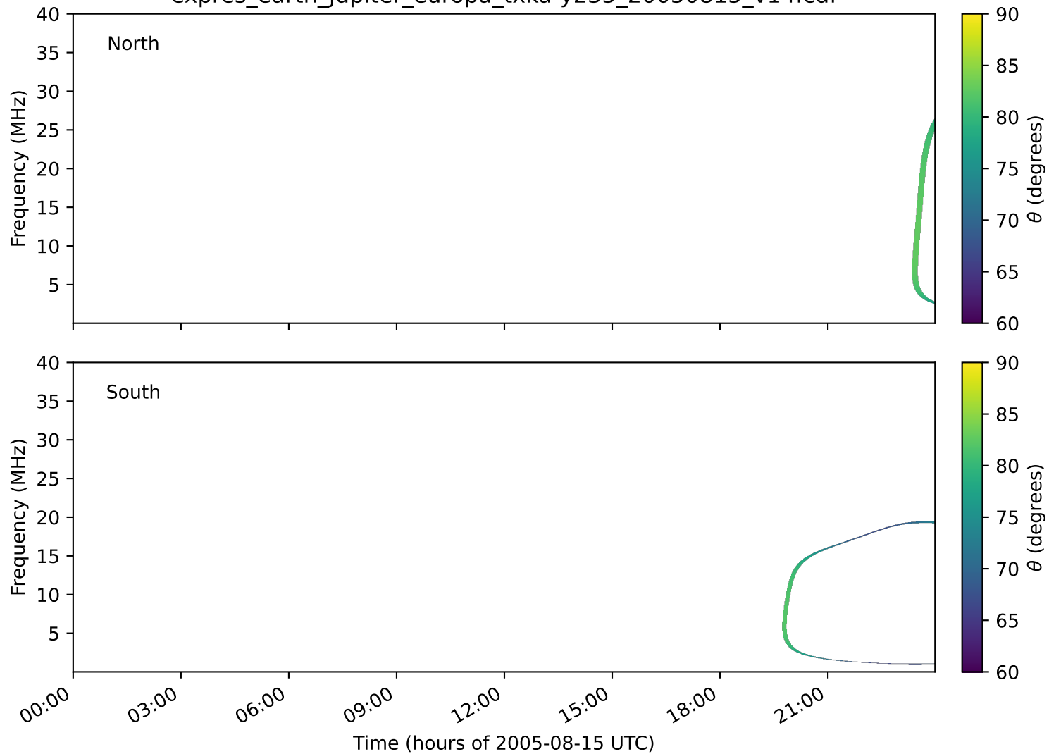
expres_earth_jupiter_europa_txka-y235_20050815_v14.cdf
