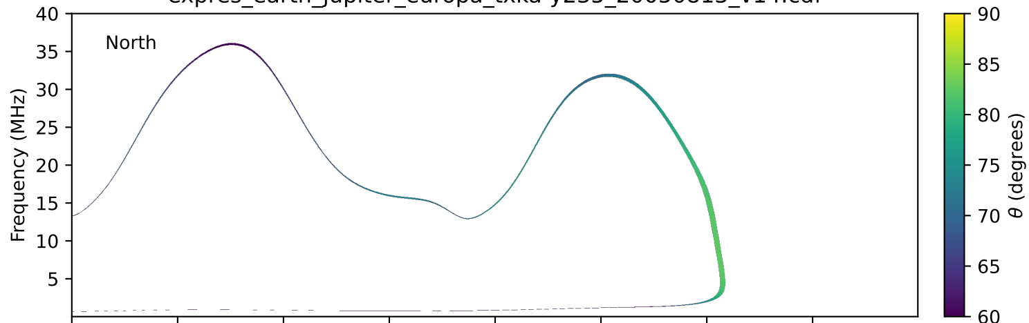
expres_earth_jupiter_europa_txka-y235_20050813_v14.cdf
