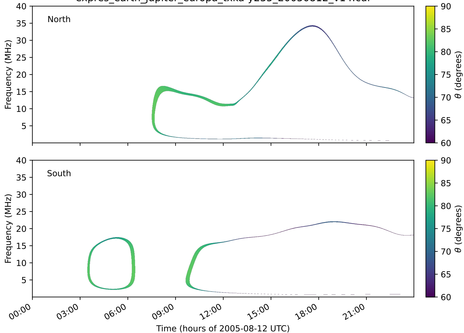
expres_earth_jupiter_europa_txka-y235_20050812_v14.cdf
