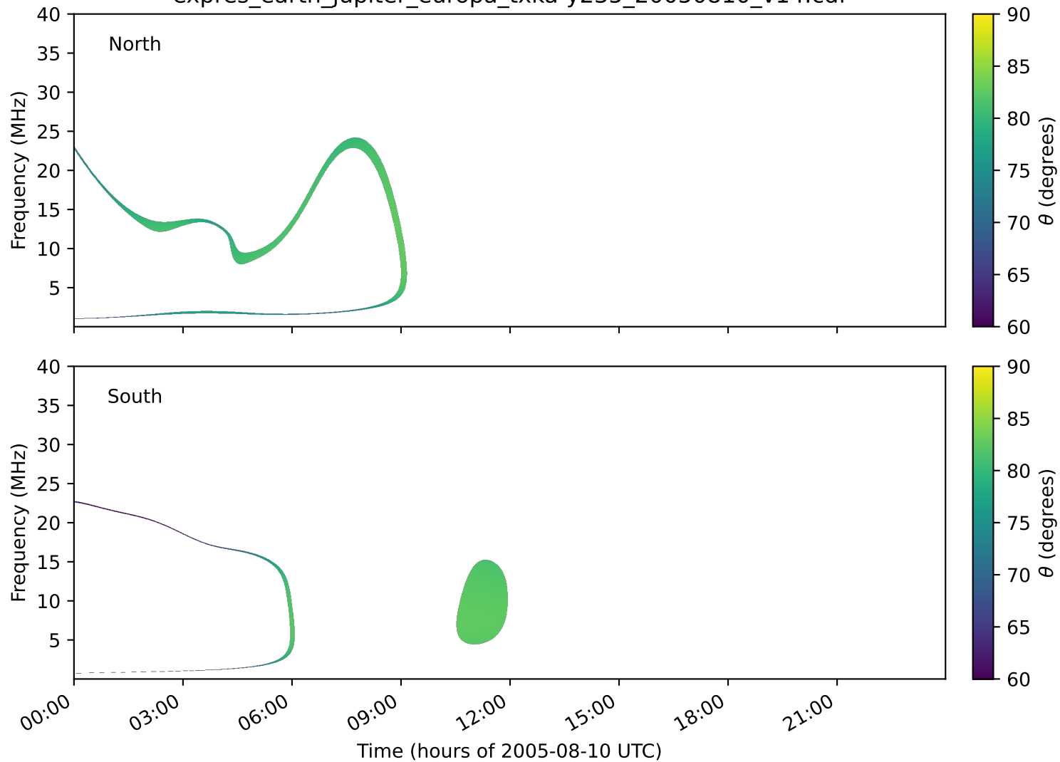
expres_earth_jupiter_europa_txka-y235_20050810_v14.cdf
