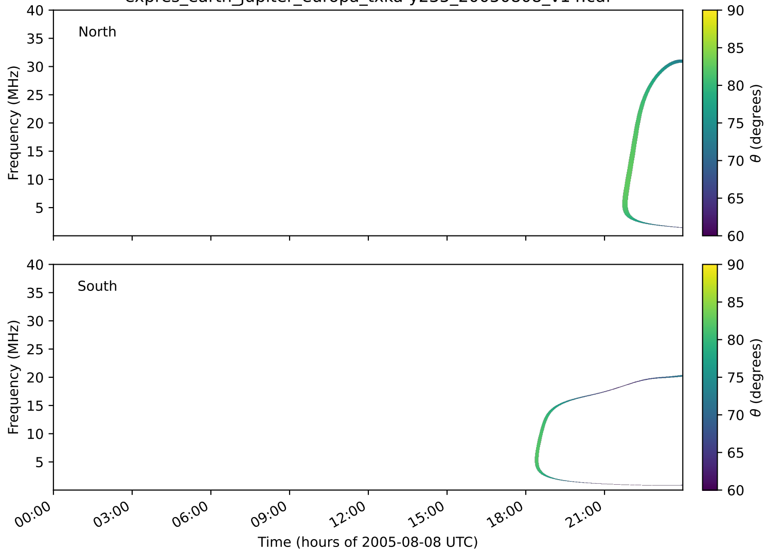
expres_earth_jupiter_europa_txka-y235_20050808_v14.cdf
