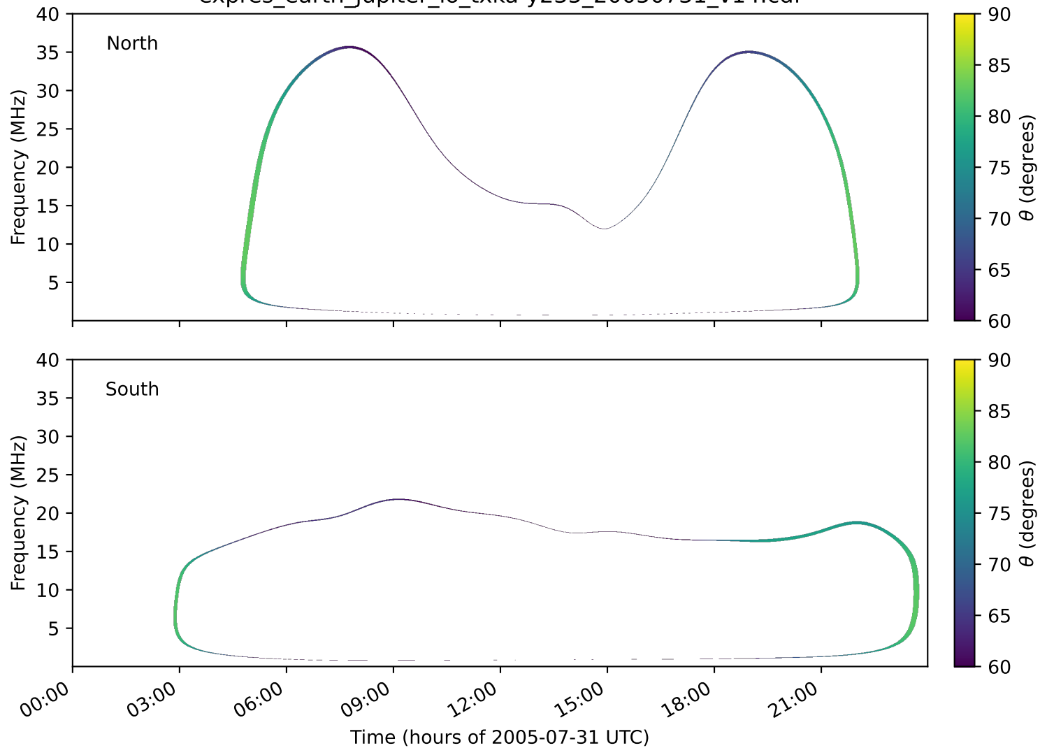
expres_earth_jupiter_io_txka-y235_20050731_v14.cdf
