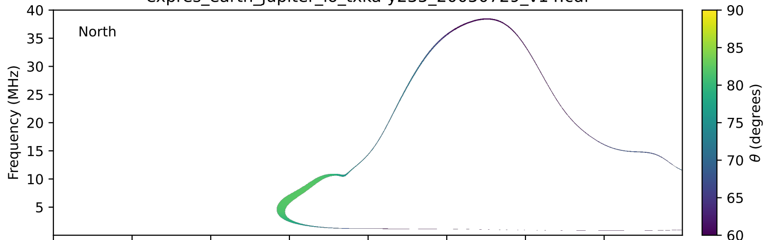
expres_earth_jupiter_io_txka-y235_20050729_v14.cdf
