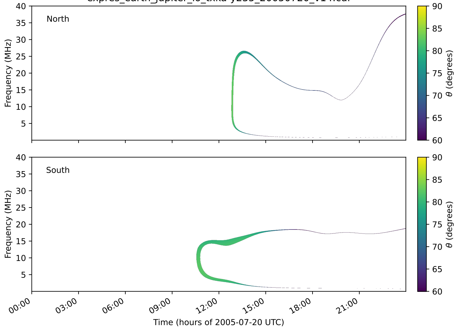
expres_earth_jupiter_io_txka-y235_20050720_v14.cdf
