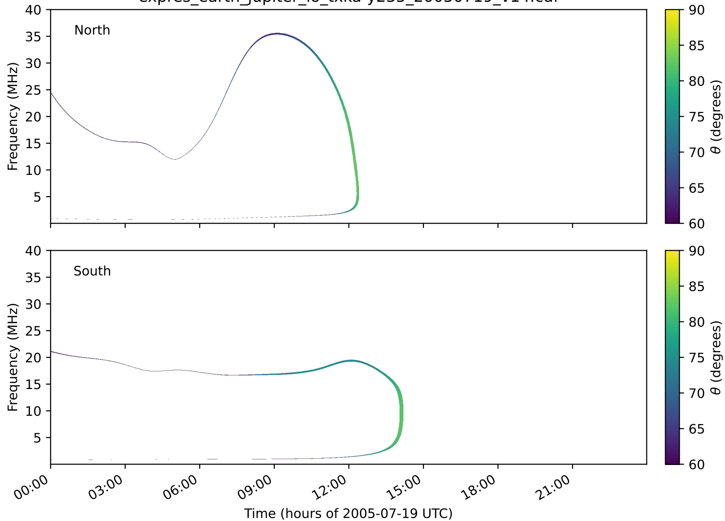
expres_earth_jupiter_io_txka-y235_20050719_v14.cdf
