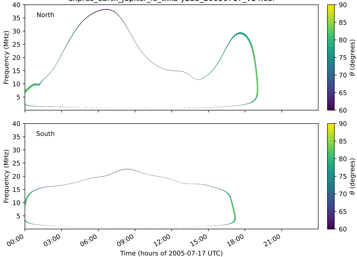
expres_earth_jupiter_io_txka-y235_20050717_v14.cdf
