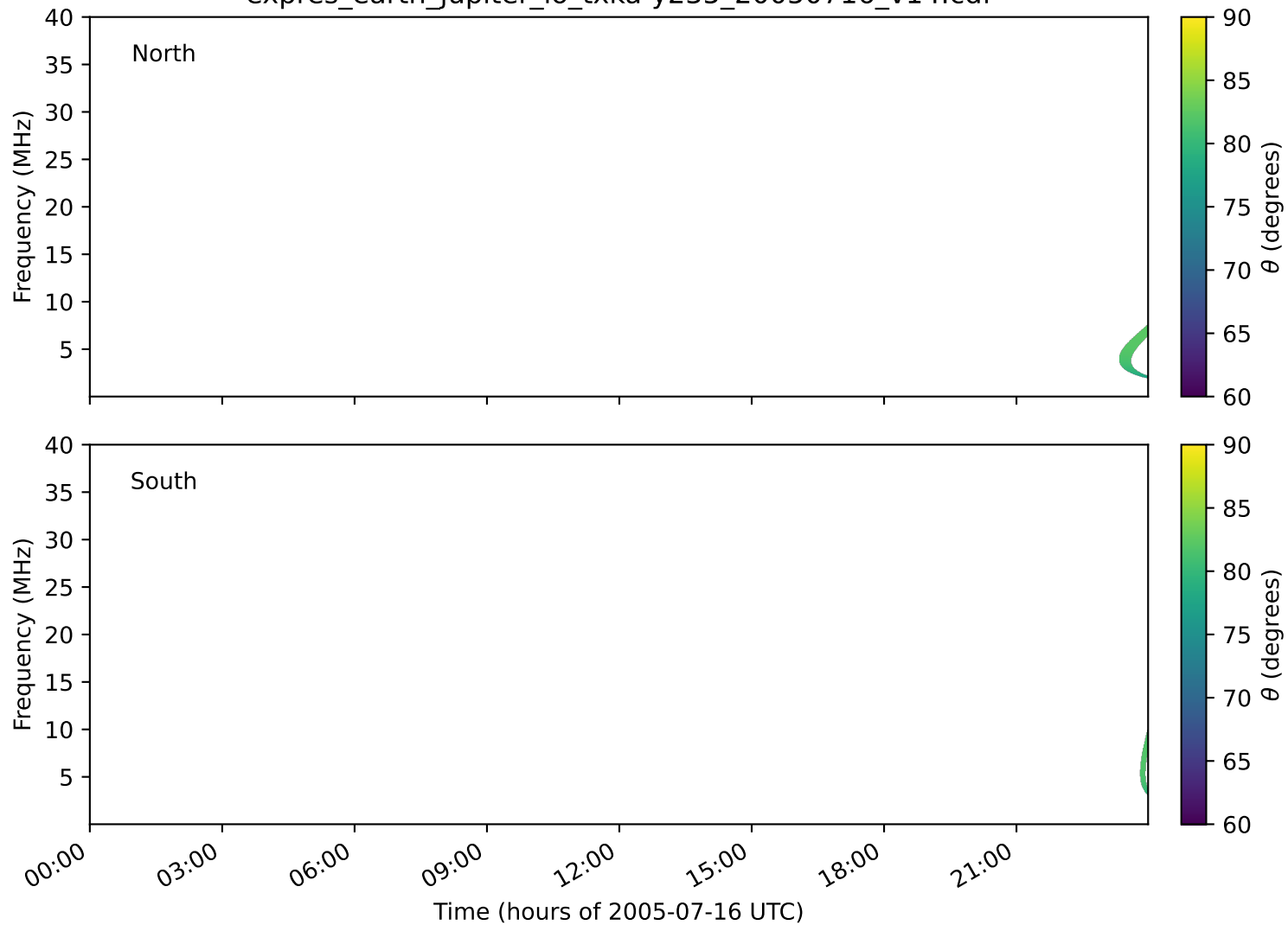
expres_earth_jupiter_io_txka-y235_20050716_v14.cdf
