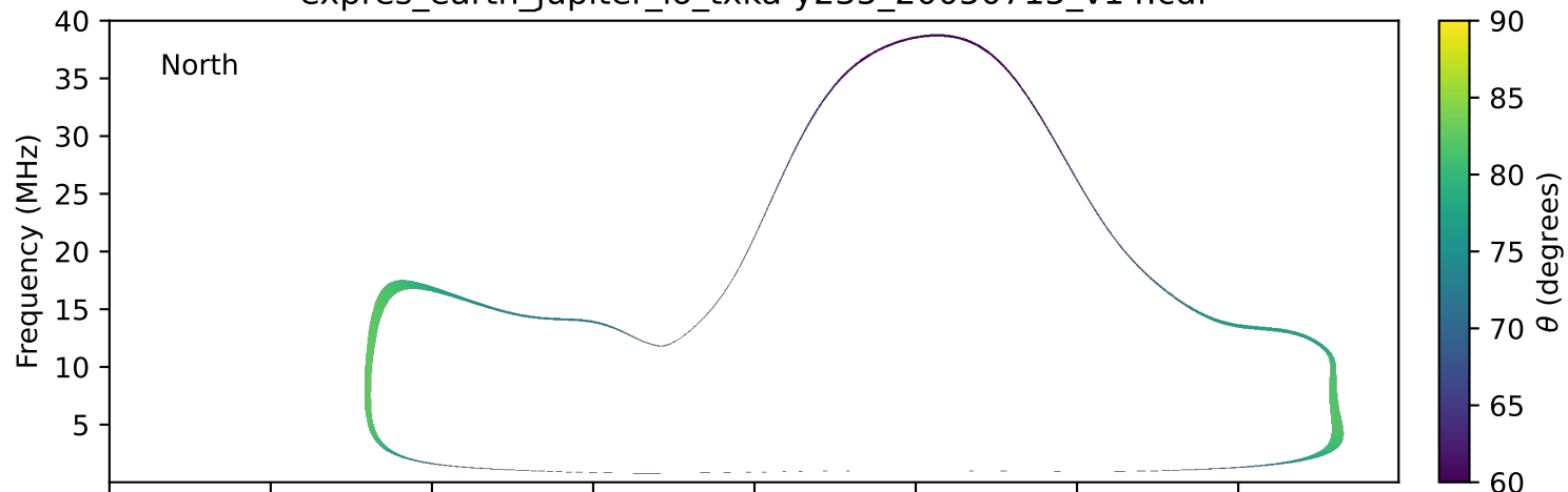
expres_earth_jupiter_io_txka-y235_20050715_v14.cdf
