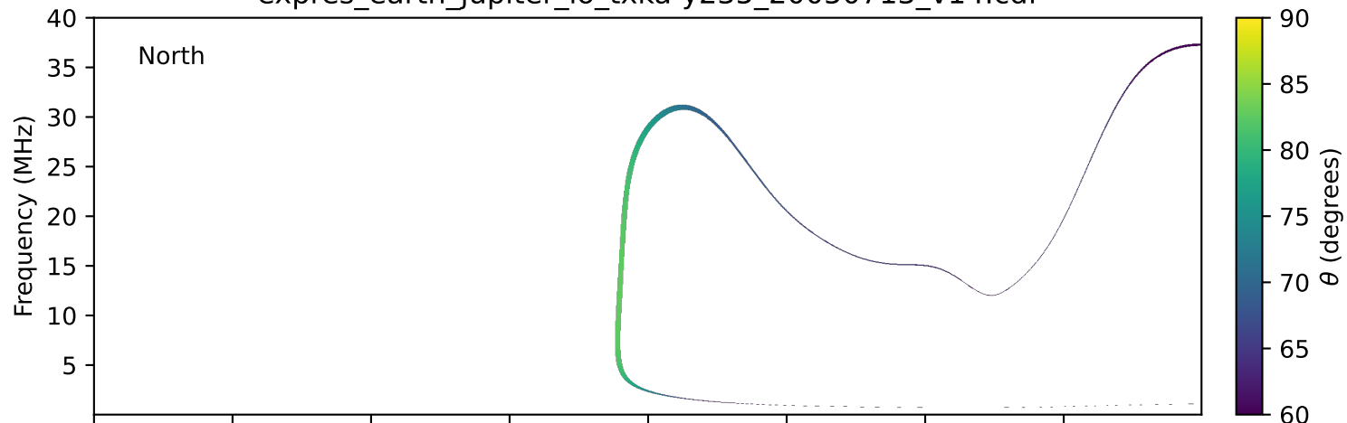
expres_earth_jupiter_io_txka-y235_20050713_v14.cdf
