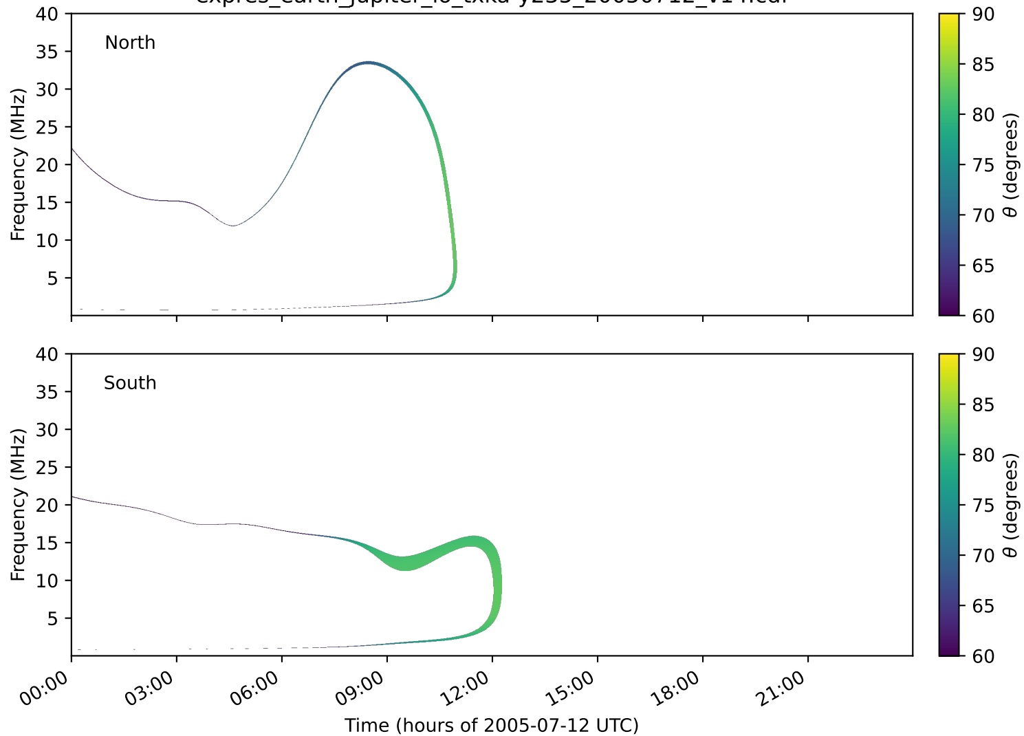
expres_earth_jupiter_io_txka-y235_20050712_v14.cdf
