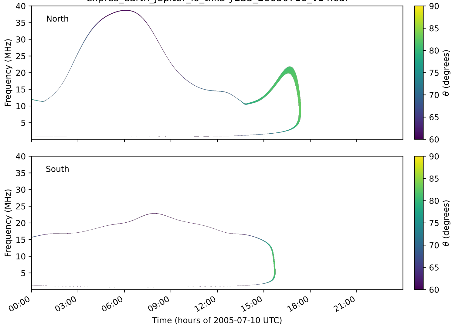
expres_earth_jupiter_io_txka-y235_20050710_v14.cdf
