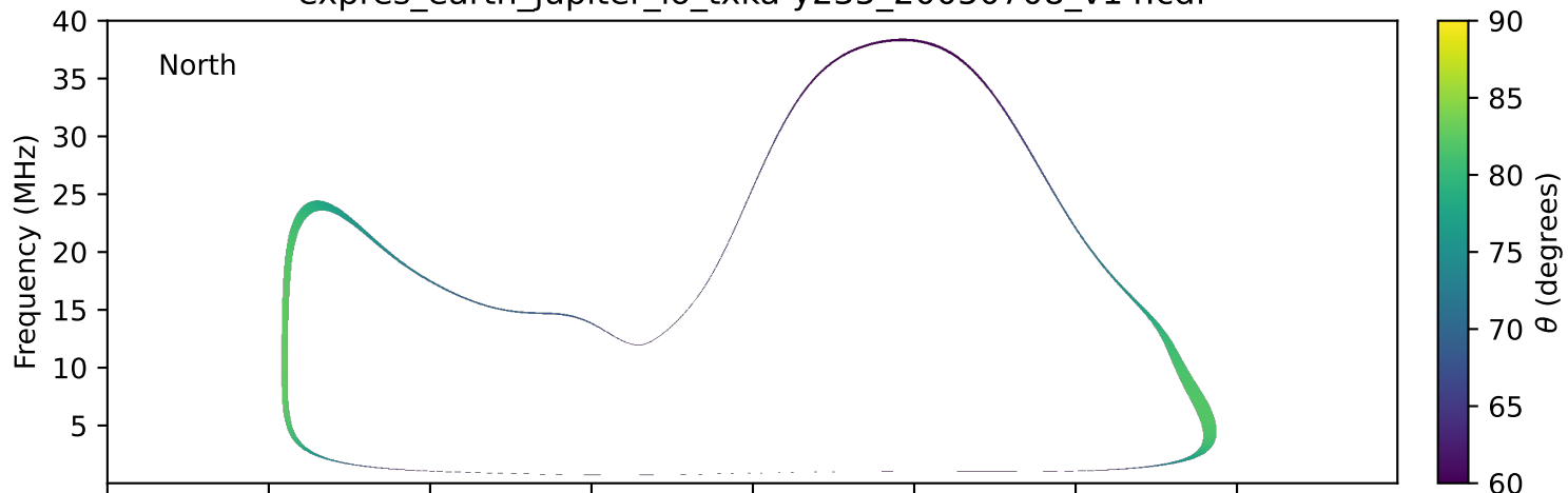
expres_earth_jupiter_io_txka-y235_20050708_v14.cdf
