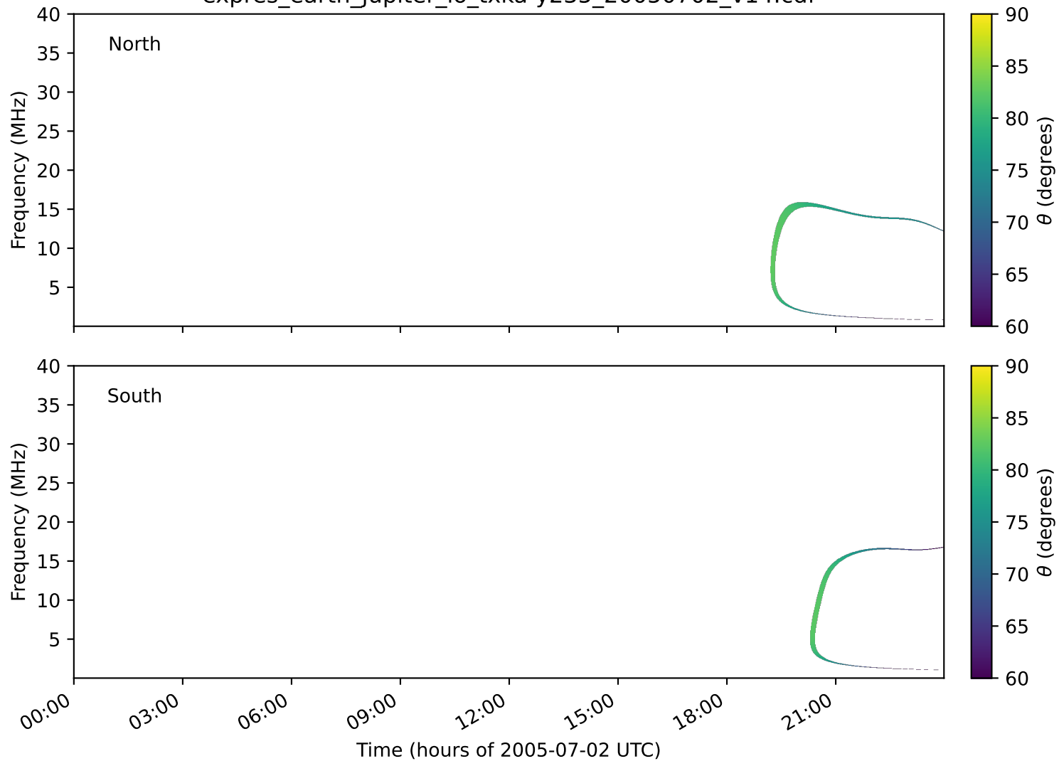
expres_earth_jupiter_io_txka-y235_20050702_v14.cdf
