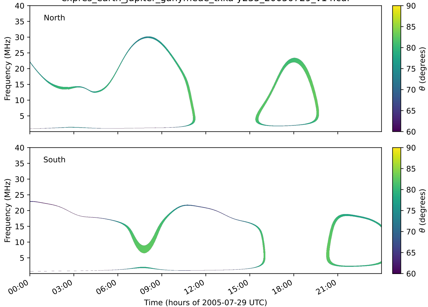
expres_earth_jupiter_ganymede_txka-y235_20050729_v14.cdf
