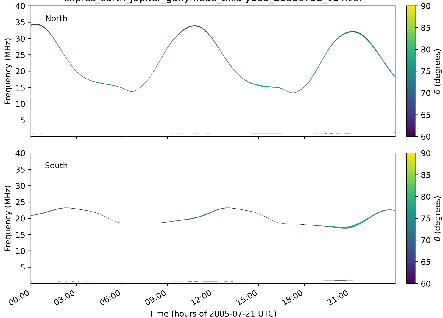
expres_earth_jupiter_ganymede_txka-y235_20050721_v14.cdf
