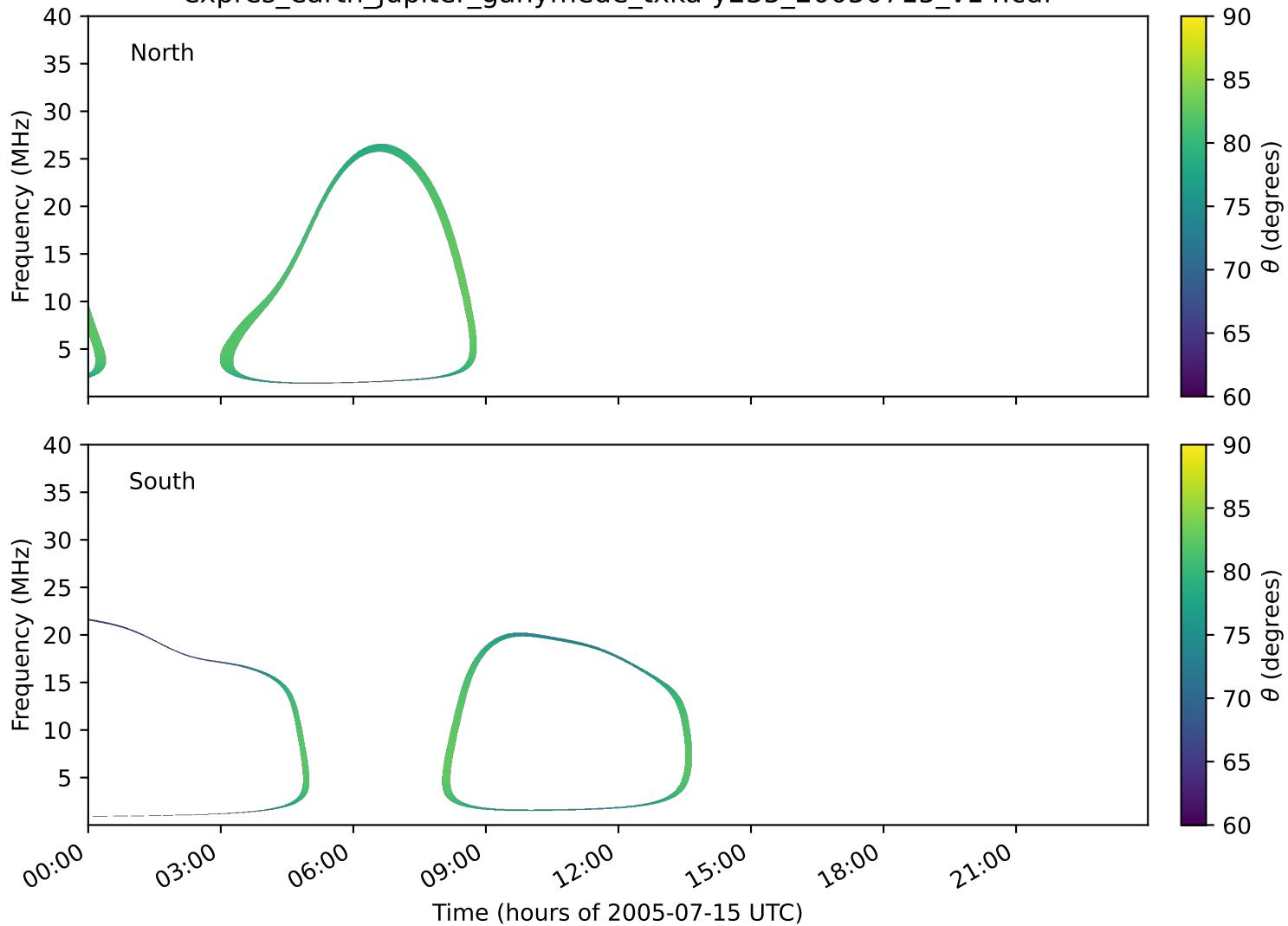
expres_earth_jupiter_ganymede_txka-y235_20050715_v14.cdf
