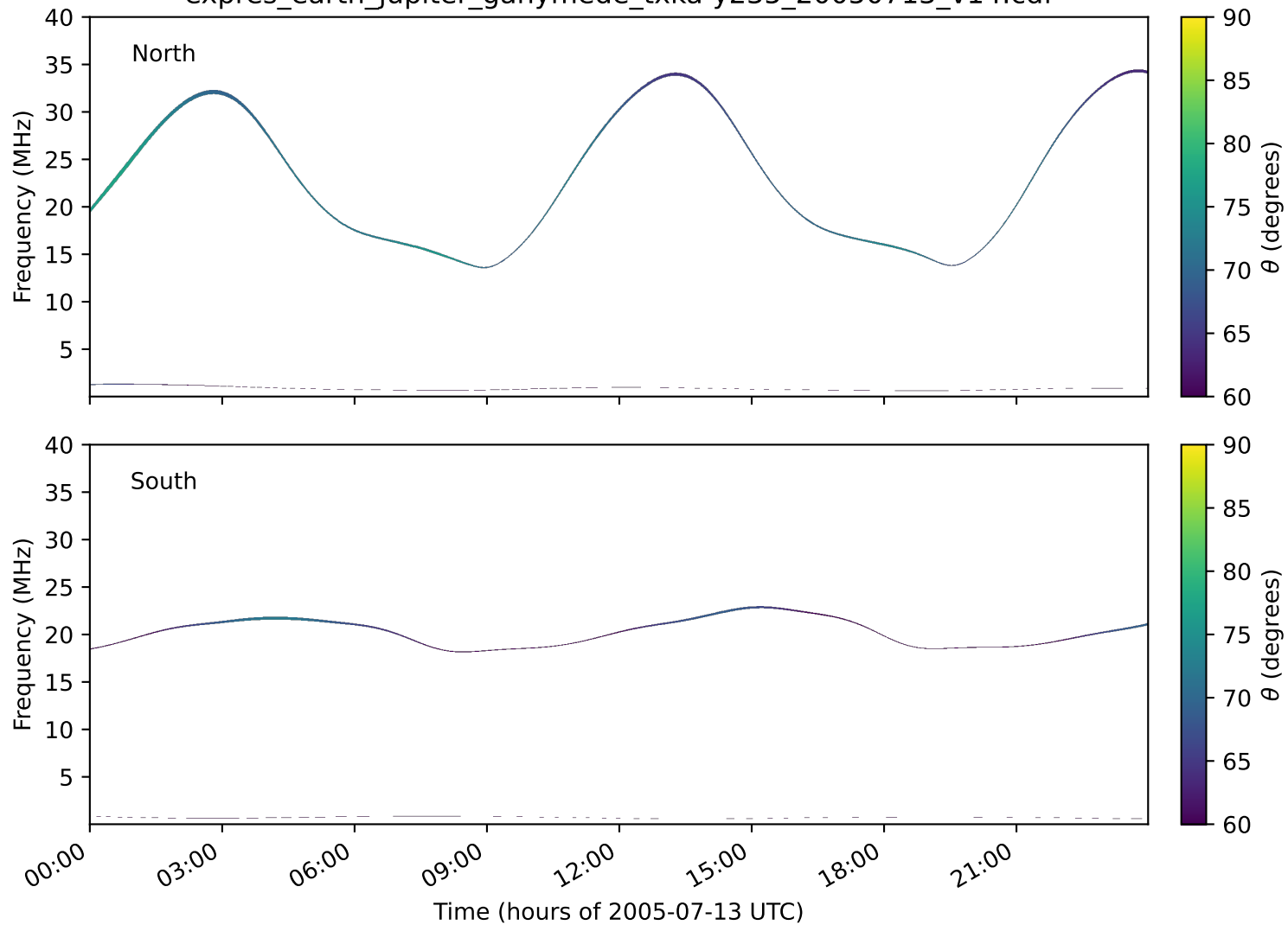
expres_earth_jupiter_ganymede_txka-y235_20050713_v14.cdf
