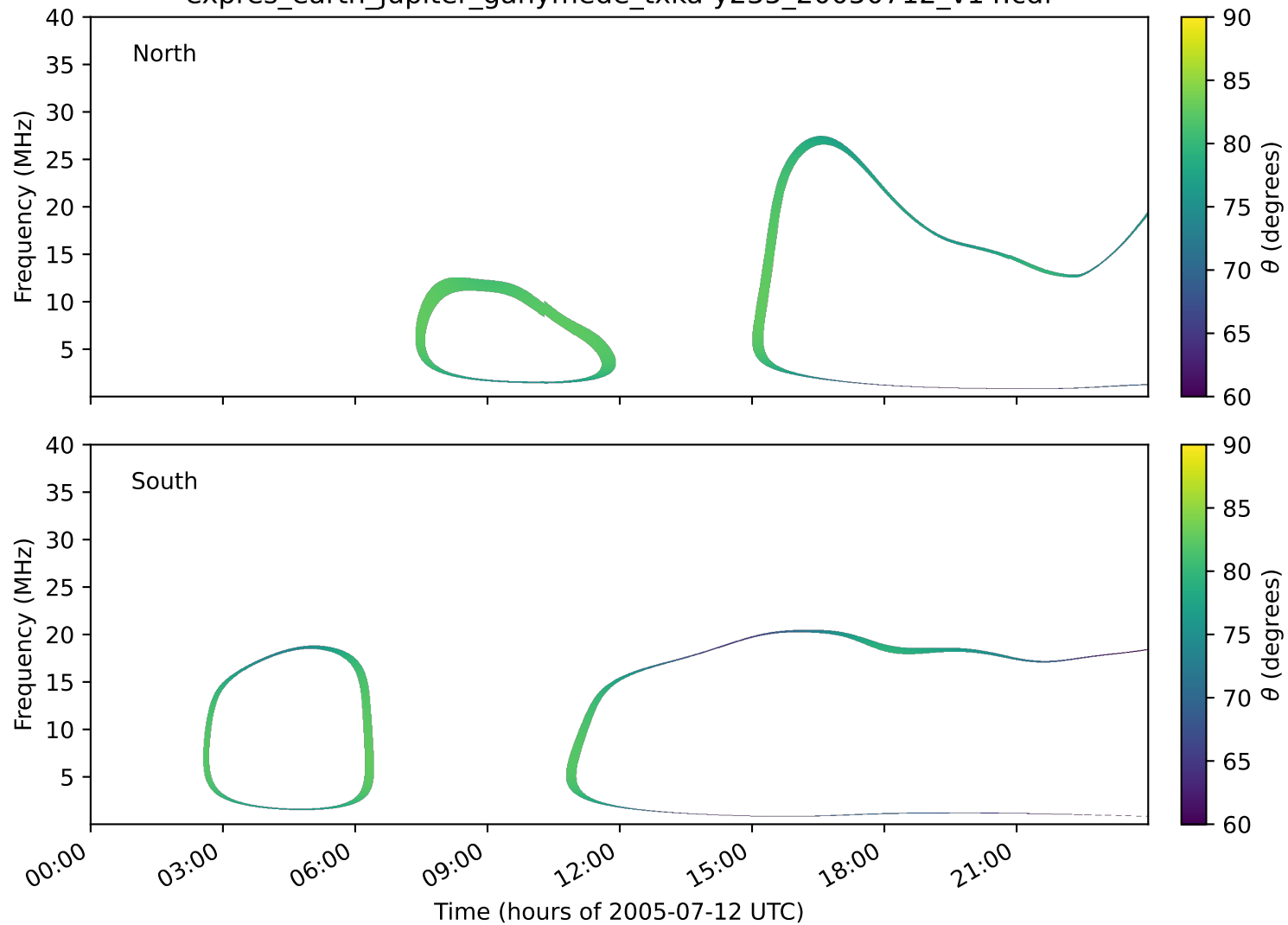
expres_earth_jupiter_ganymede_txka-y235_20050712_v14.cdf
