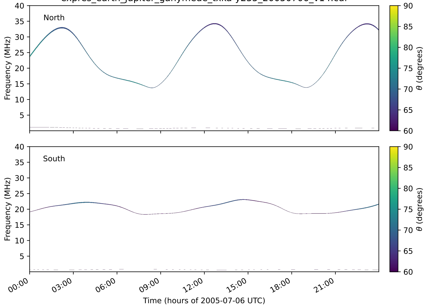
expres_earth_jupiter_ganymede_txka-y235_20050706_v14.cdf
