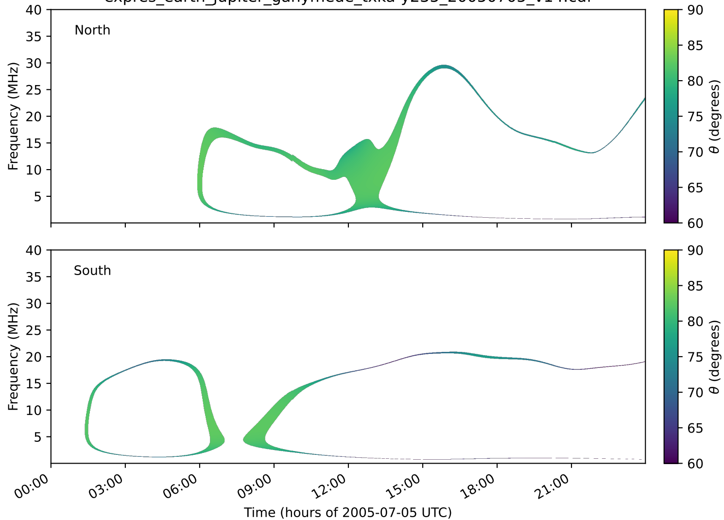
expres_earth_jupiter_ganymede_txka-y235_20050705_v14.cdf
