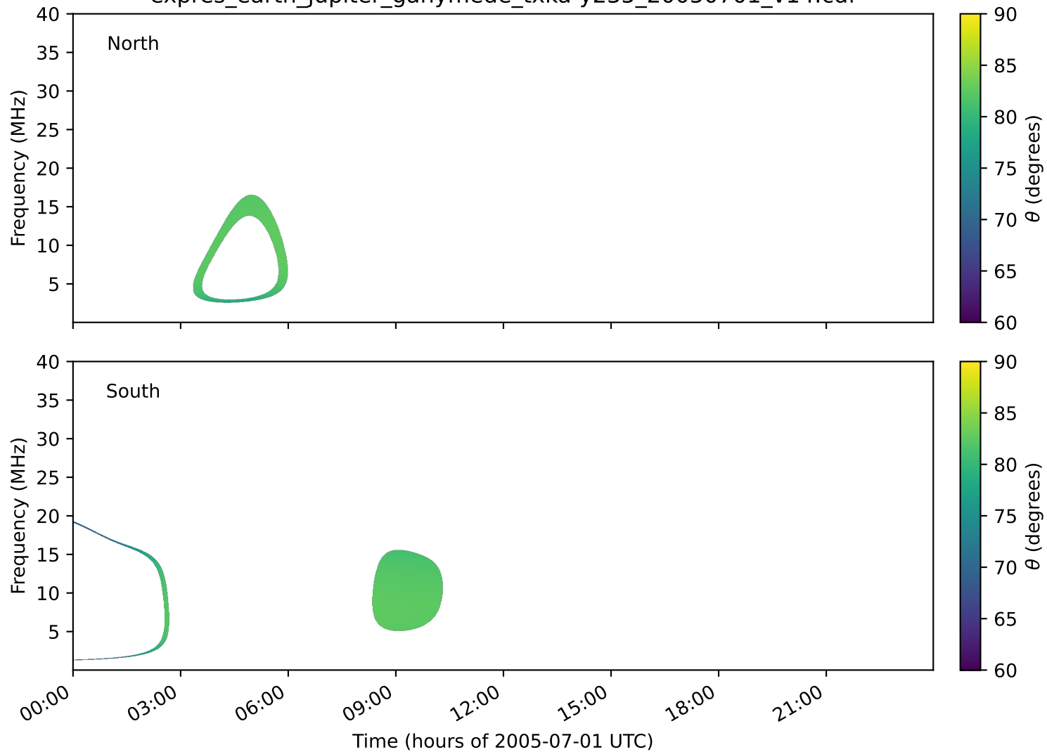
expres_earth_jupiter_ganymede_txka-y235_20050701_v14.cdf
