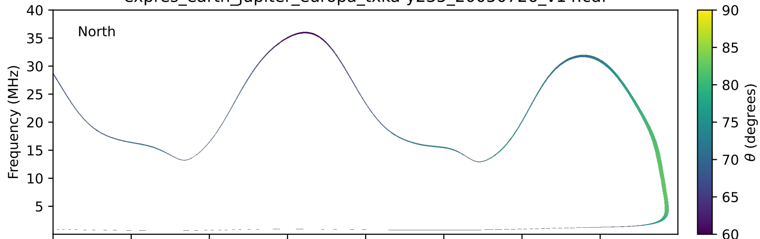
expres_earth_jupiter_europa_txka-y235_20050726_v14.cdf
