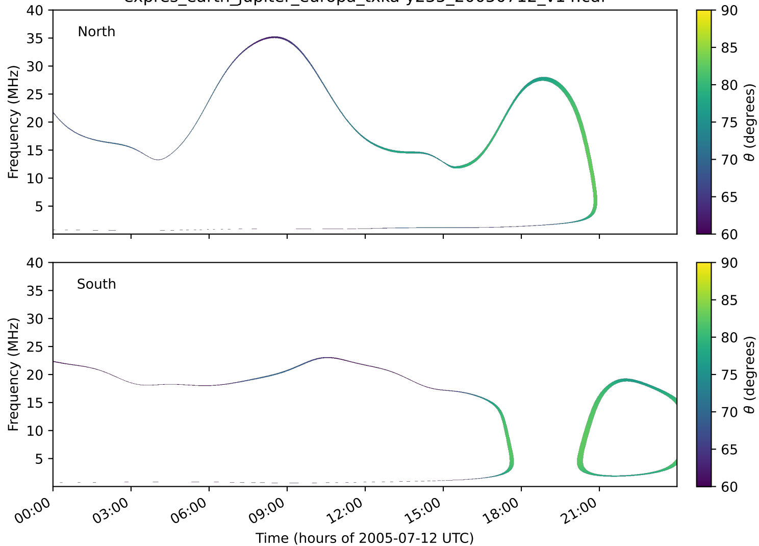
expres_earth_jupiter_europa_txka-y235_20050712_v14.cdf
